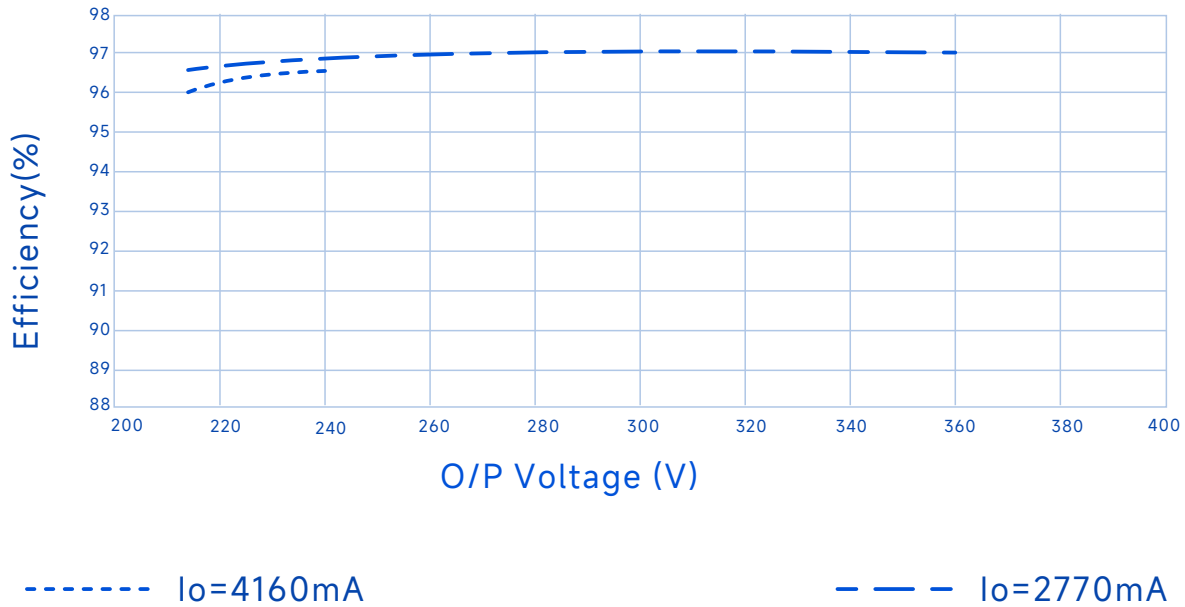
Efficiency Vs. O/P Voltage ( V_{in}=220V_{ac} )
