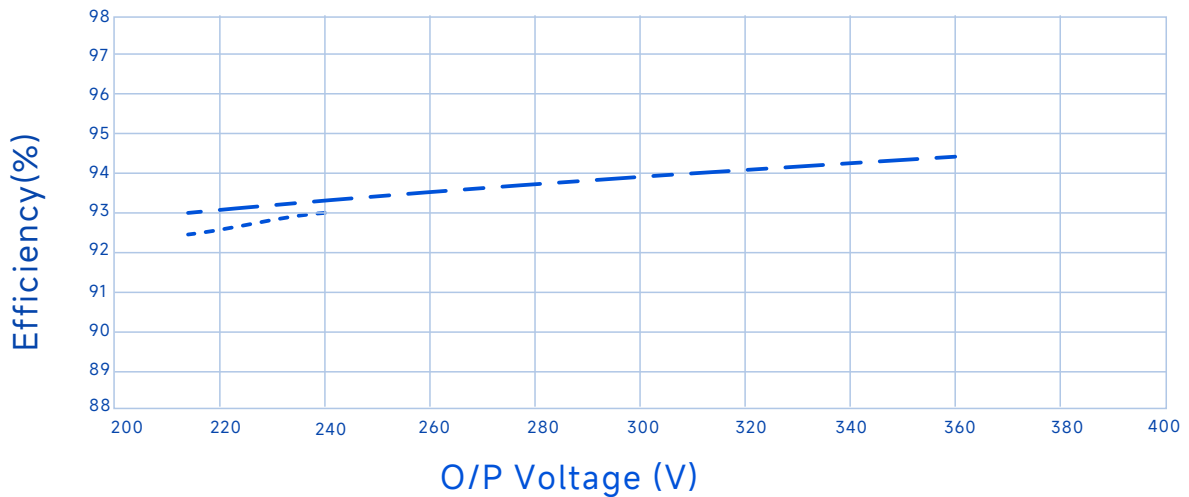
Efficiency Vs. O/P Voltage (Vin=120Vac)
